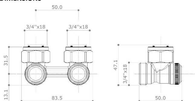
(3/4"x18) X (3/4"x18) 0925 inclus
